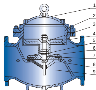
FIG.2-Piston type
